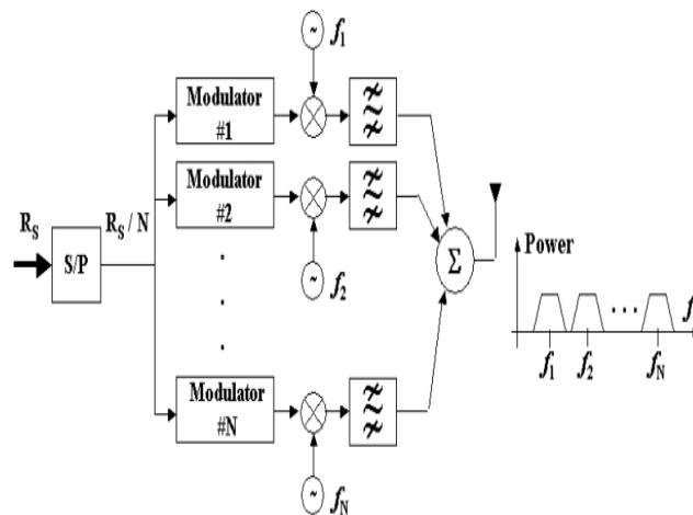
FIGURE 2.1: Block Diagram of MCM transmitter.
